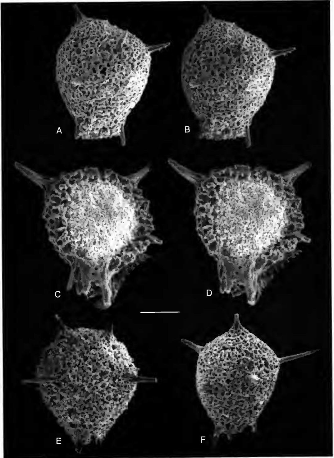
FIG. 12. — Glomeropyle grantmackiei Aita, n. sp.; A, B, paratype, stereograph (photo Nos 31066, 31067); C, D, stereograph (photo Nos 31098, 31097); E, (photo No. 31072); F, paratype (photo No. 31073). Sample YABC-26, Bull Creek, Caples Terrane, Otago, South Island. Scale bar: 100 \mu m.
